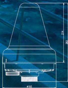
Sketch of antenna ADU camouflage
