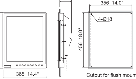
Cutout for flush mount
