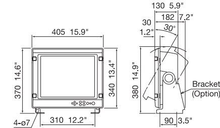
MU-151C Bracket Mount 8.6 kg 20.1 lb
