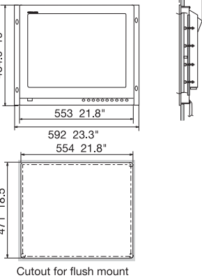
Cutout for flush mount
