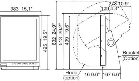
MU-190V Bracket Mount 11.0 kg 24.3 lb
