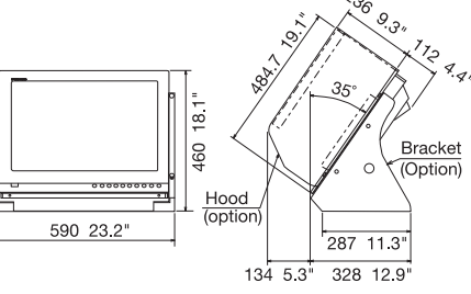
MU-231 Bracket Mount 18.9 kg 41.7 lb
