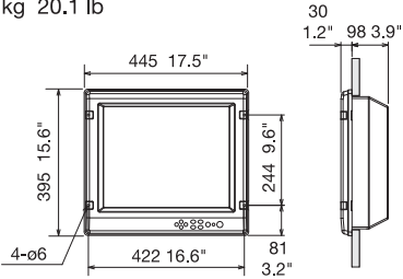
MU-170C Flush Mount 7.5 kg 20.1 lb
