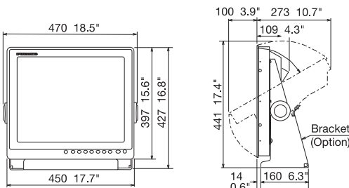
MU-190HD Bracket Mount 11 kg 24.3 lb
