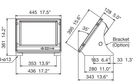
MU-170C Bracket Mount 12.9 kg 32 lb
