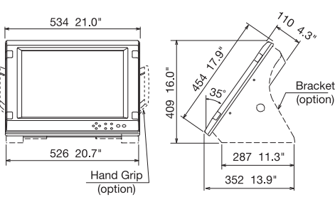
MU-201C Bracket Mount 17.0 kg 37.5 lb
