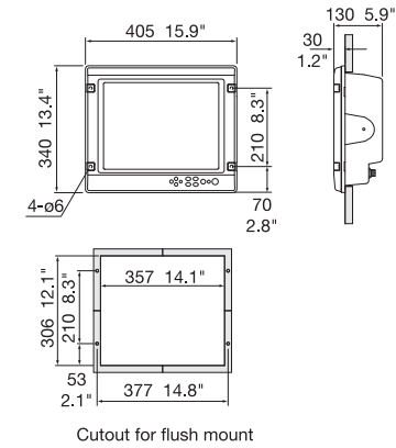
Cutout for flush mount
