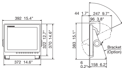
MU-150HD Bracket Mount 7.4 kg 16.3 lb
