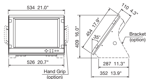
MU-231 Flush Mount 12.8 kg 28.2 lb
