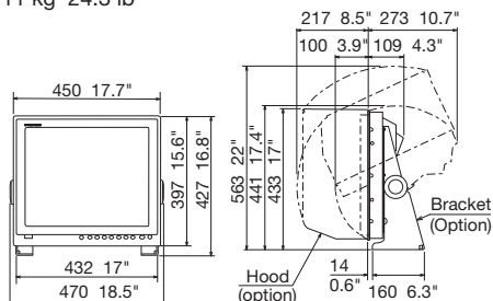
MU-190 Bracket Mount 11 kg 24.3 lb
