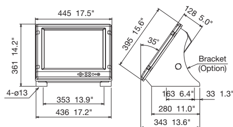
MU-190V Flush Mount 8.0 kg 17.6 lb
