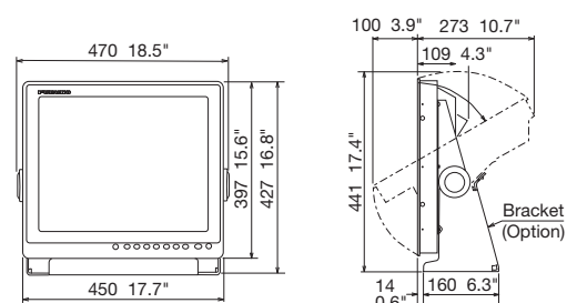
MU-190HD Bracket Mount 11 kg 24.3 lb
